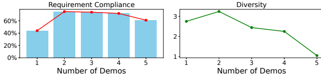
Fig. 13: As the number of Demos increases, the success rate in Requirement Compliance and Diversity initially rises and then decreases.
